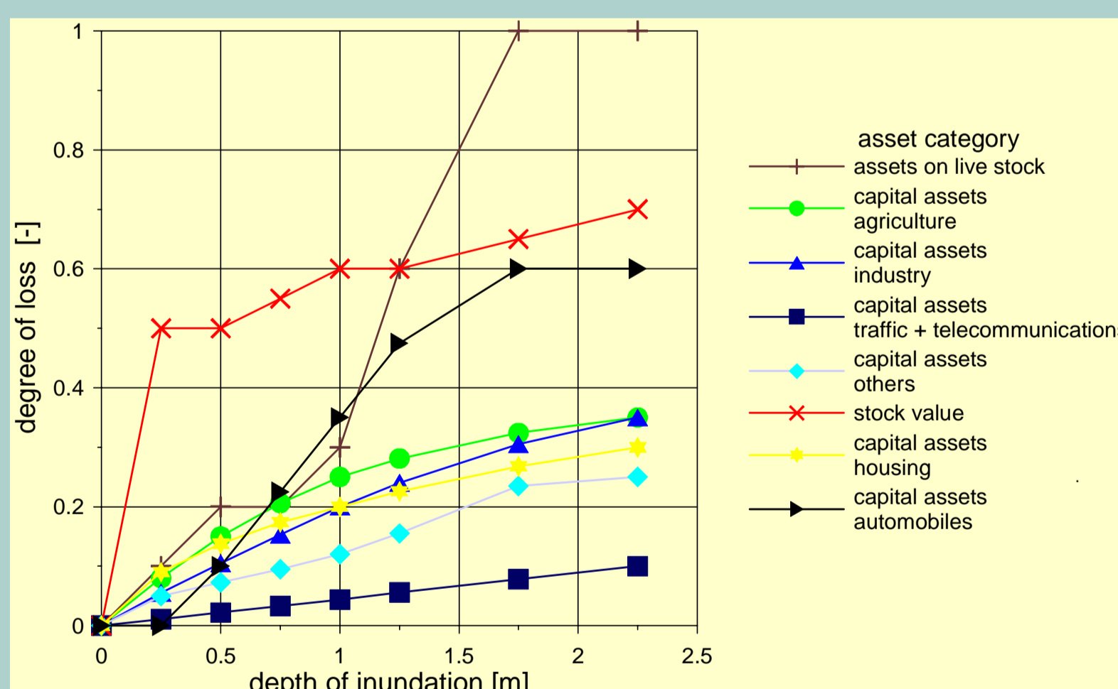
Figure 5: Loss functions for different asset categories (based on Klaus & Schmidtke)
