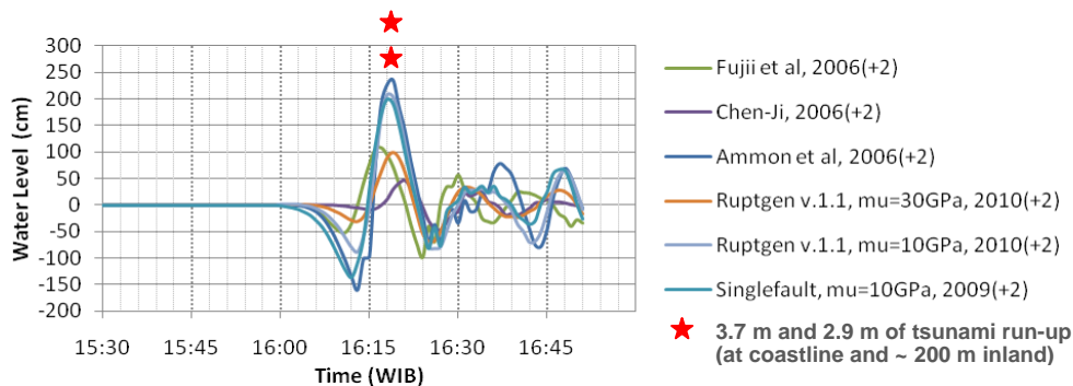
Figure 11. Marigram vs. water level at witness location in cilacap (109.089E, 7.691S)
