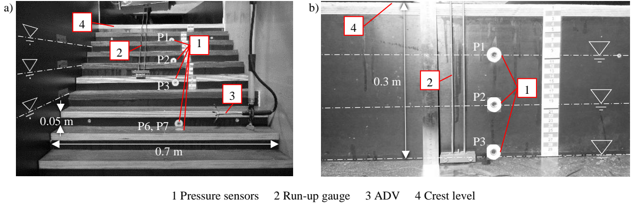
Figure 2. Impression of the model set-up with instrumentation for a) step height 0.05 m and b) step height 0.3 m.
