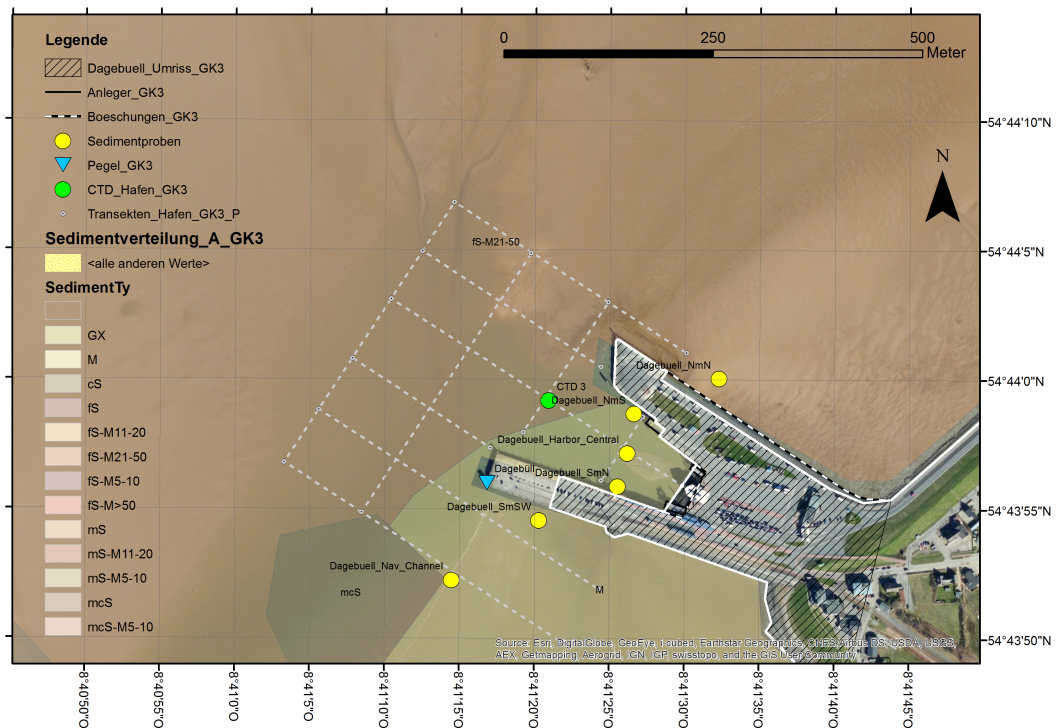
Figure 1: Measurement plan for the Port of Dagebüll including ADCP-transects, CTD-profile locations, soil sample positions and occurring sediment types
